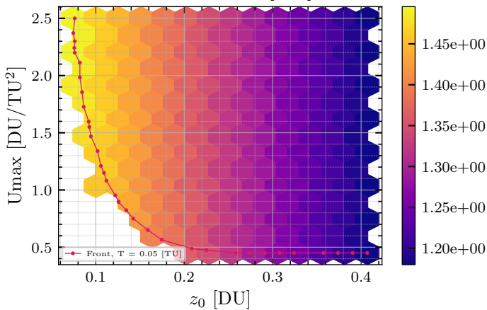
Period = 0.05 [TU]
