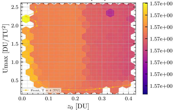
Period = 4 [TU]
